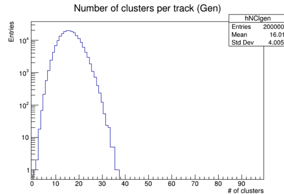
Clusters number distribution, for a muon at 10 GeV traversing 200 cells, 1 cm per side, filled with 10% He and 90 % iC4H10, simulated with Garfield ++ .
