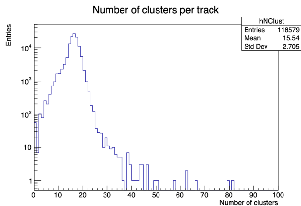
Clusters number distribution, for a muon at 10 GeV traversing as simulated with GEANT 4 IDEA full SIM framework .
