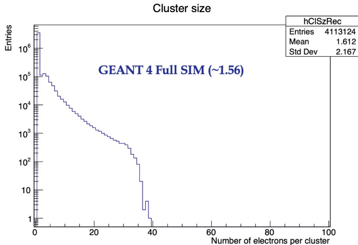
Cluster size distribution, for a muon at 10 GeV
