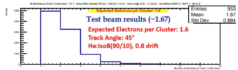
Electron per Clusters Distribution
