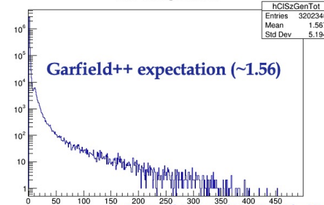
Electron per Clusters Distribution
