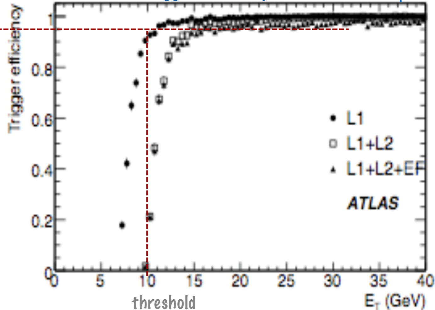
ATLAS: e10 trigger efficiency as a function of E_T
