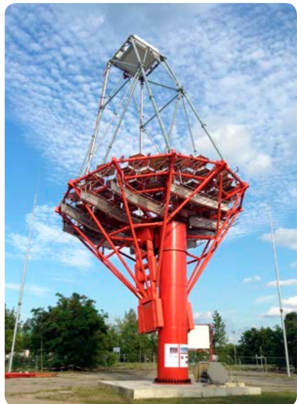
Cherenkov Telescope Array prototype (Credit: CTA)
