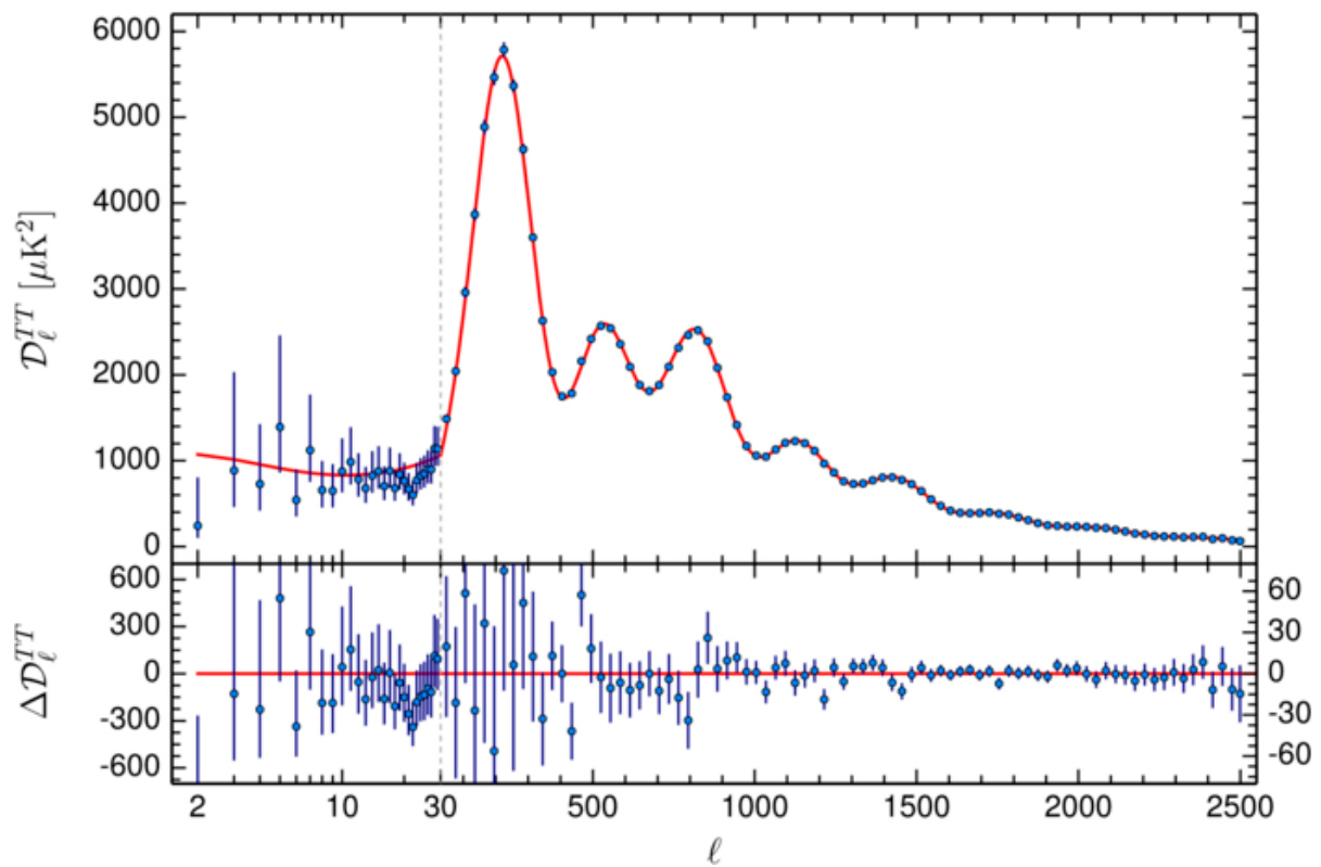
Planck power spectrum (Credit: ESA)
