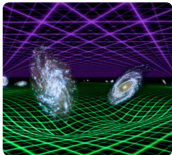
In this artist's conception, dark energy is represented by the purple grid above, and gravity by the green grid below. Gravity emanates from all matter in the universe, but its effects are localised and drop off quickly over large distances. Credit: NASA/JPL-Caltech
