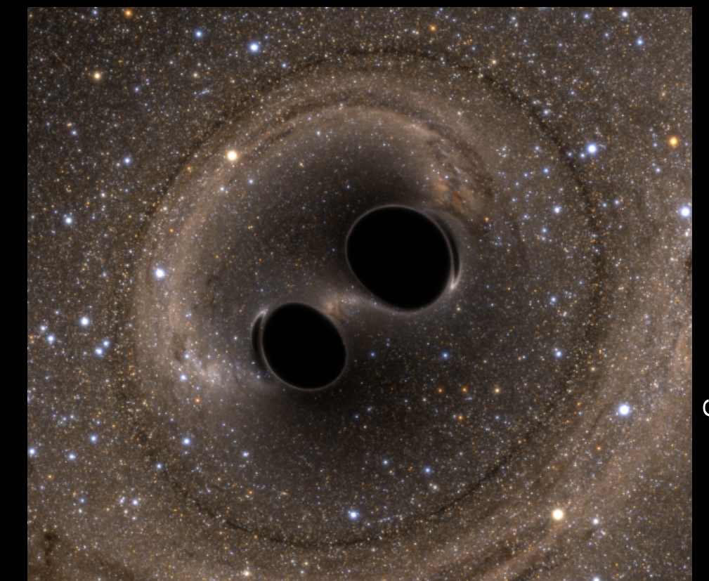
BH/NS Mergers
