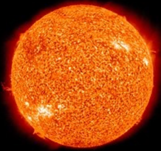
The Sun
