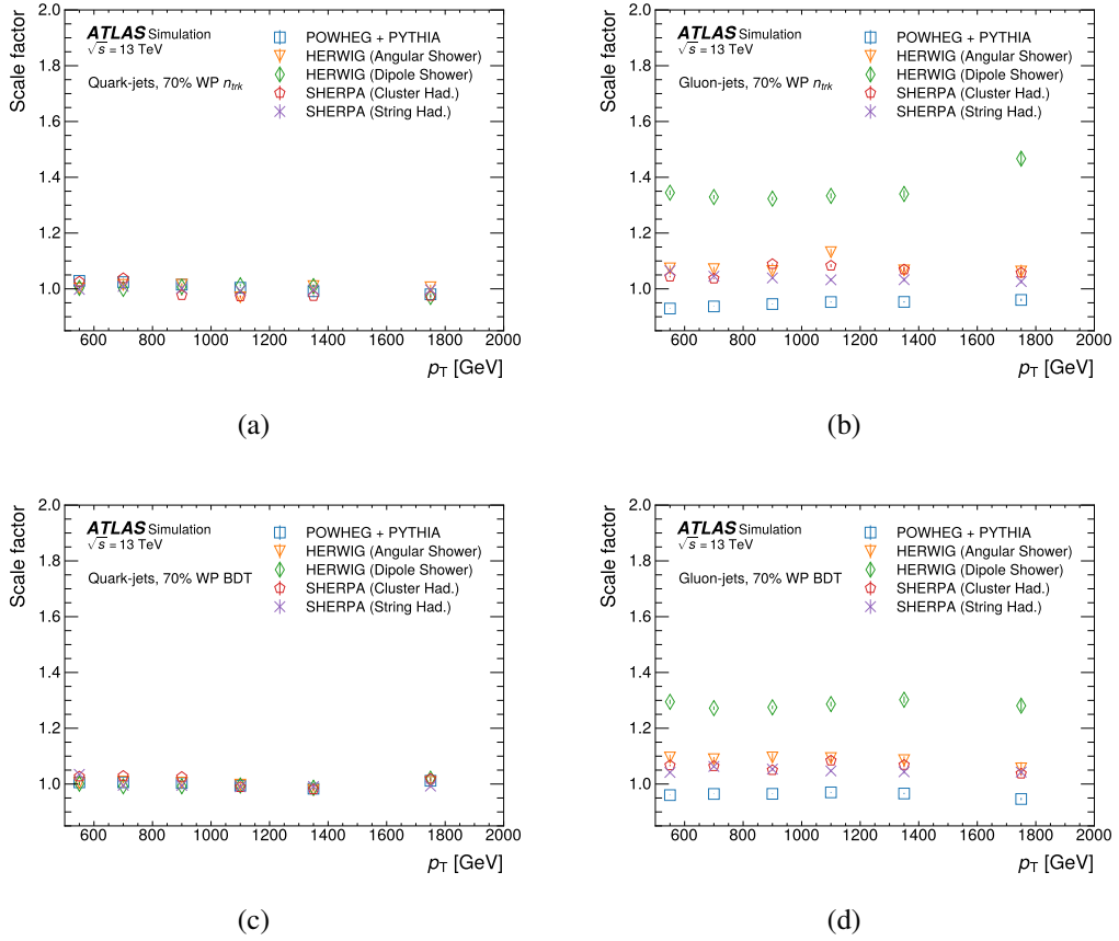
Figure 5.45 The MC-to-MC SF of the N_{trk} , (a) and (b), and BDT, (c) and (d), as a function of jet p_T for quark-jets (left) and gluon-jets (right) at the 70% WP. The vertical error bars show the statistical uncertainty.
