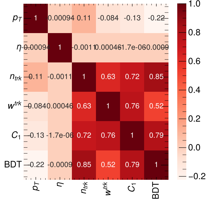
Figure 5.16 correlation matrix of jet variables.
