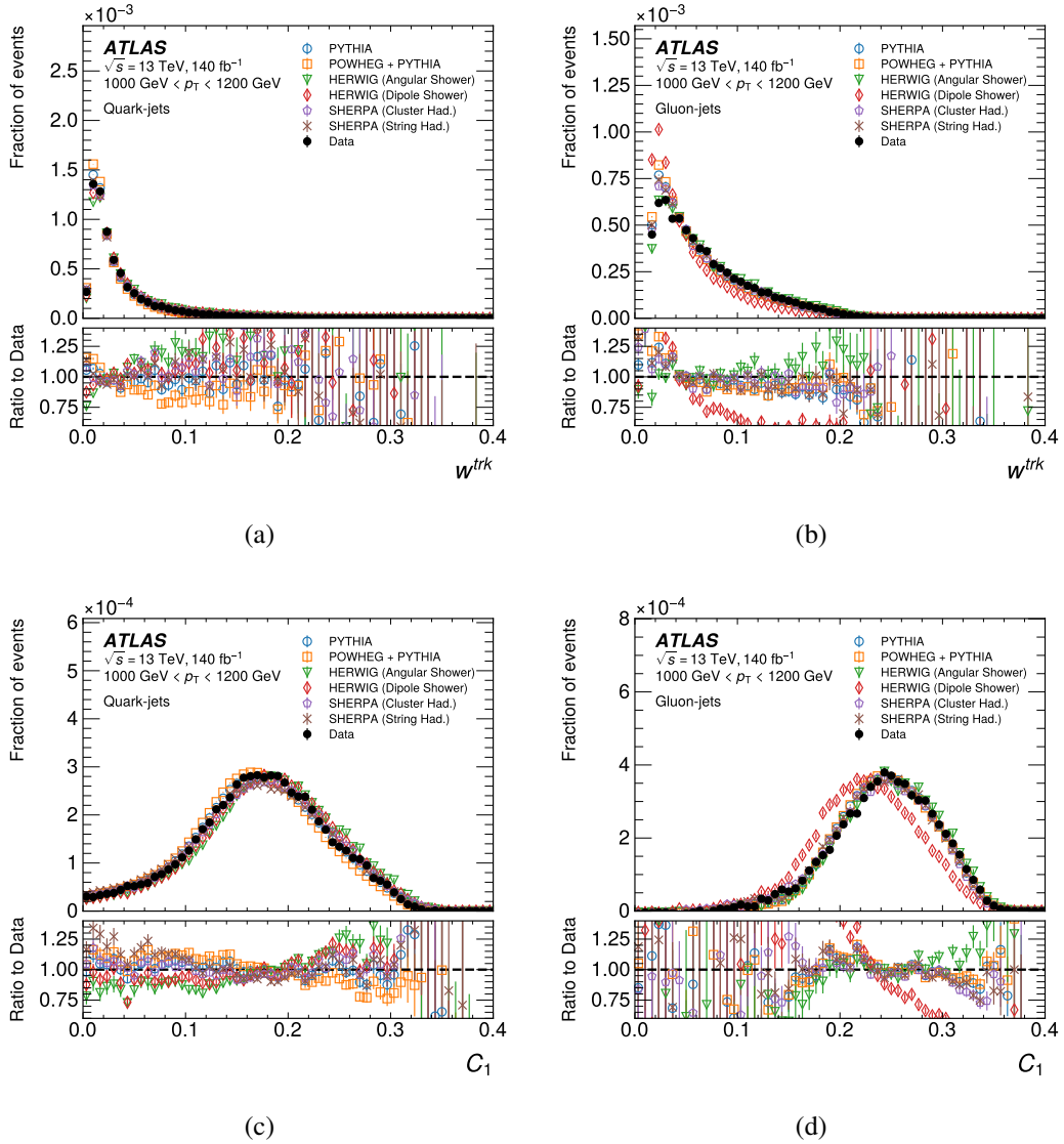
Figure 5.32 The distributions of W_{\text{trk}} (a,b) and C_1 (c,d) for quark-jets (left) and gluon-jets (right) using different generators (open symbols) and data (closed symbol) are shown in the upper panels. The lower panels show the ratio of each MC distribution and the data. The vertical error bars show the statistical uncertainty.
