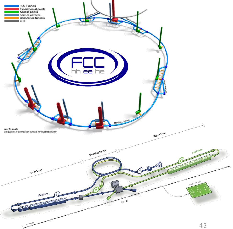
FUTURE CIRCULAR COLLIDER (FCC) - 3D Schematic Underground Infrastructure - Single Tunnel Design John Osborne - Charlie Cook - Angel Navascués
