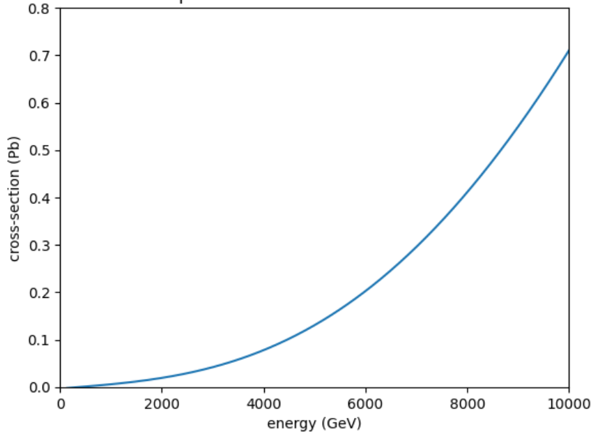
polarized muon W cross-section
