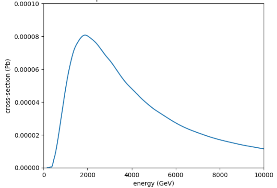
polarized muon Z cross-section
