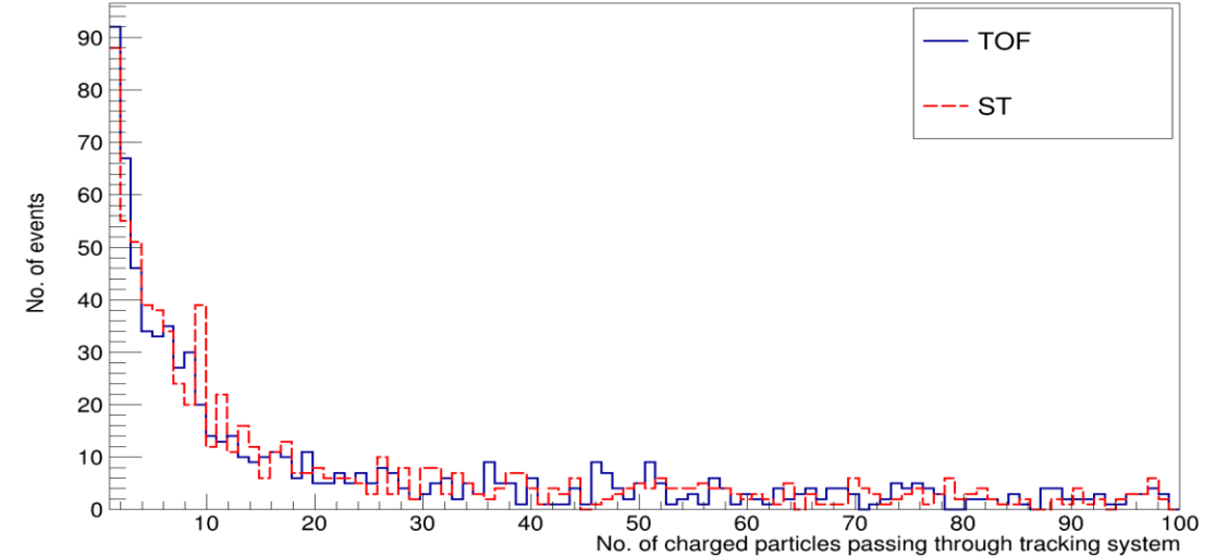
Total multiplicity of charged particles passing through tracking system, Ca40-Ca40
