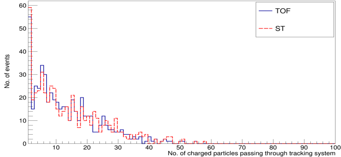
Total multiplicity of charged particles passing through tracking system, C12-C12
