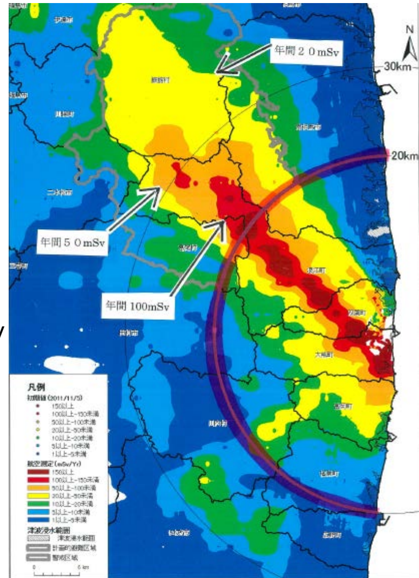
Predicted annual dose (as of 2011Nov5) [SOURCE] http://www.meti.go.jp/earthquake/nuclear/pdf/111226_01a.pdf
