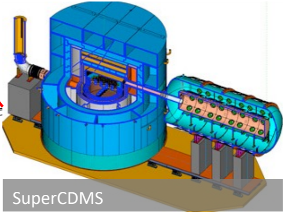
NEWS-G
