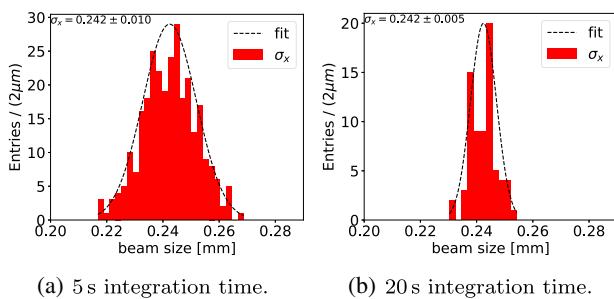
FIG. 14. Distribution of independent beam size measurements for two integration times. Black lines are fits with a normal distribution, whose width reflects the statistical error of the BGV beam size measurement.
