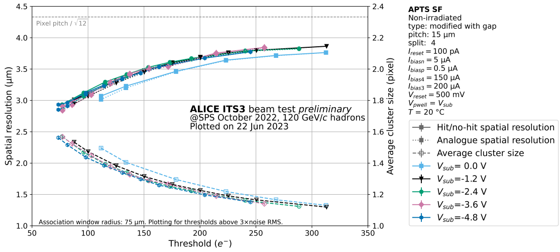
Figure 1: Hit/no-hit spatial (solid lines) and analogue (dashed) resolution vs threshold at different reverse bias values V_{\text{sub}} , for a modified-with gap 15 \mu\text{m} pitch size Analogue Pixel Text Structure, reference variant.
