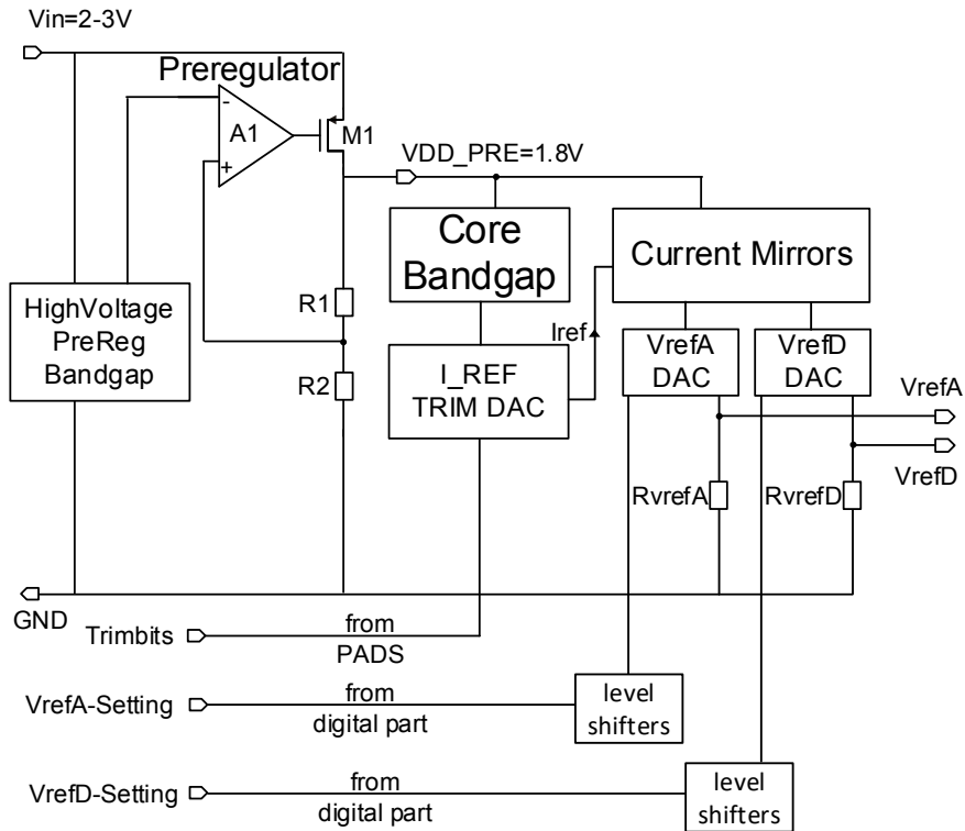
Figure 1 : The LDO architecture used in OBELIX
