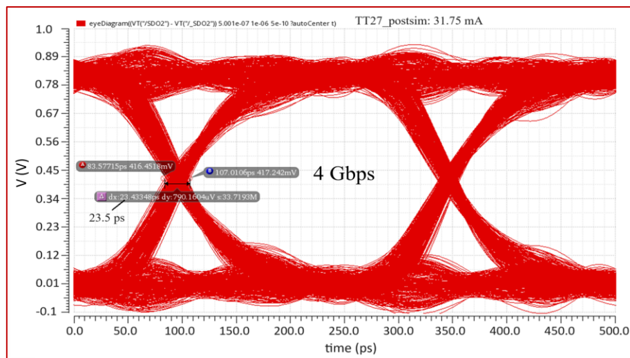
Fig. 3. Eye diagram simulation of the revision
