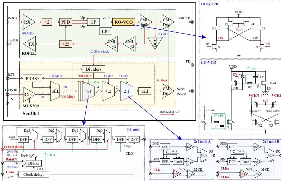
Fig. 1. Schemes of the 4 Gbps serializer prototypes
