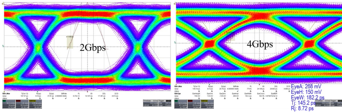
Fig. 2. Measurements of the serial data outputs of Ser20t1 (2.6 V)
