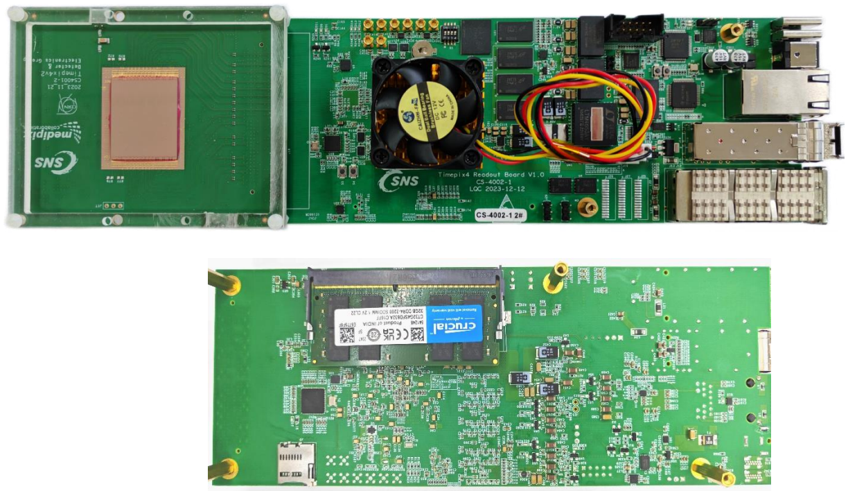
Figure 2 Prototype of Readout Electronics Based on Timepix4
