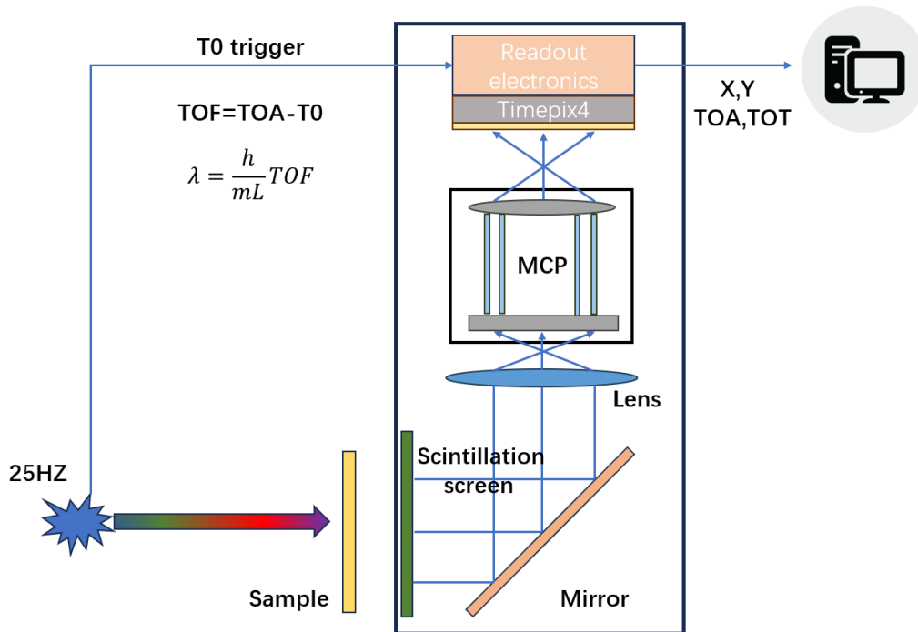
Figure 1 Diagram of Energy-Resolved Neutron Imaging Detector at CSNS
