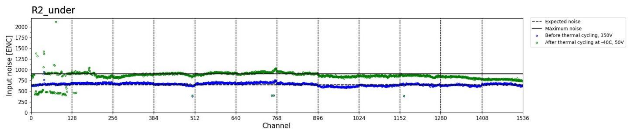
Figure 2: Input noise for a subset of the input channels of an end-cap module. The noise is compared before thermal cycling and after five thermal cycles at -40\text{ }^{\circ}\text{C} . The noise induced by sensor cracking is visible on the left-hand side of the module.
