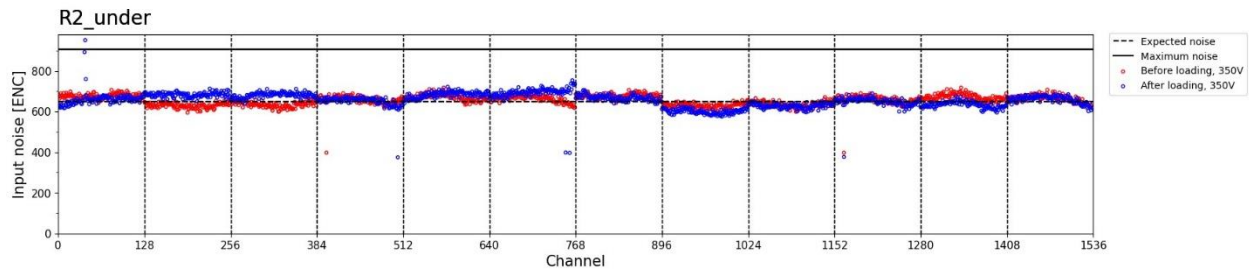
Figure 1: Input noise (units: equivalent noise charge or ENC) for a subset of the input channels of an end-cap module. The noise is compared before and after loading.
