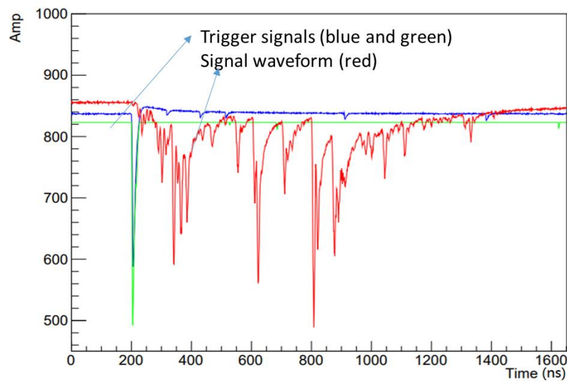
Figure 3 Typical signal acquired with the demonstrator pre-amp
