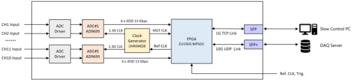
Figure 4 Block diagram of the prototype digitization electronics
