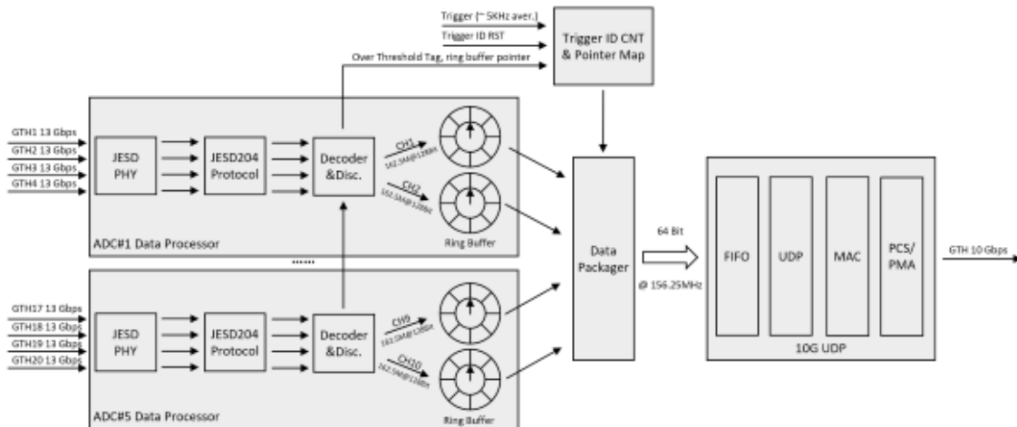
Figure 5 Block diagram of the firmware for the prototype digitization electronics
