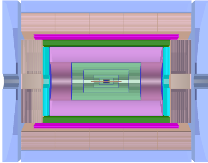
Figure 1 Detector of the main Experiment in CEPC CDR
