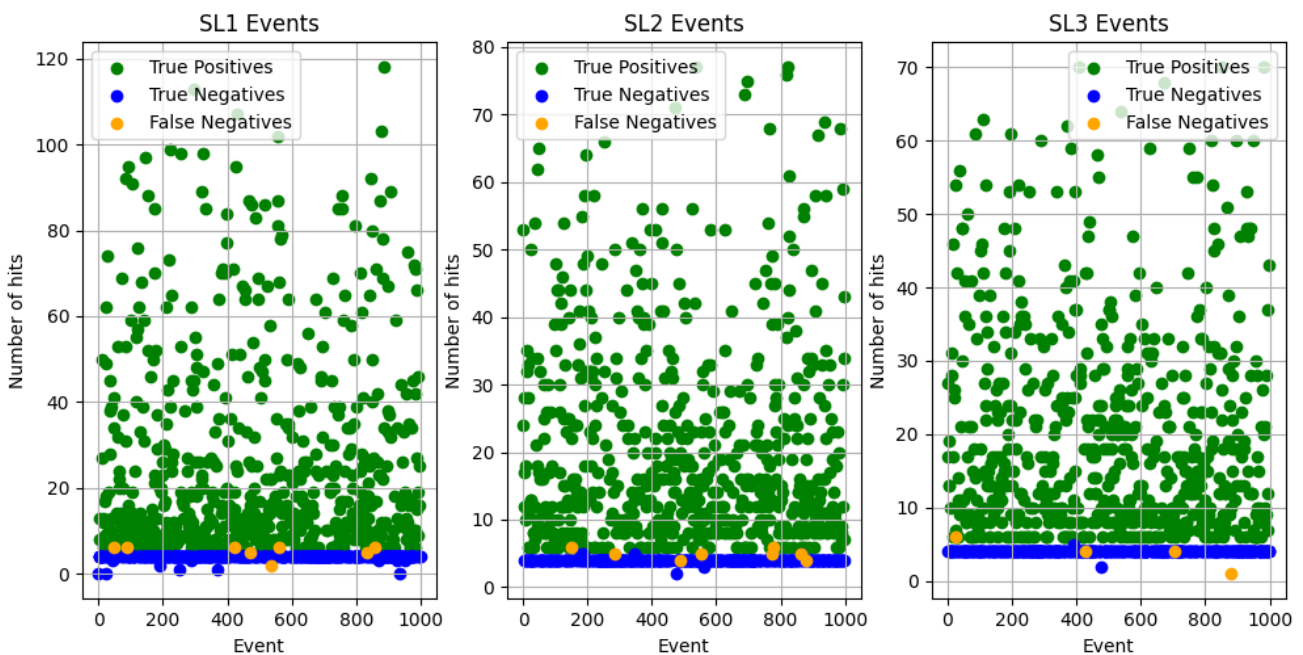
Number of hits in each event, labeled by identification result and separated by Super Layers.
