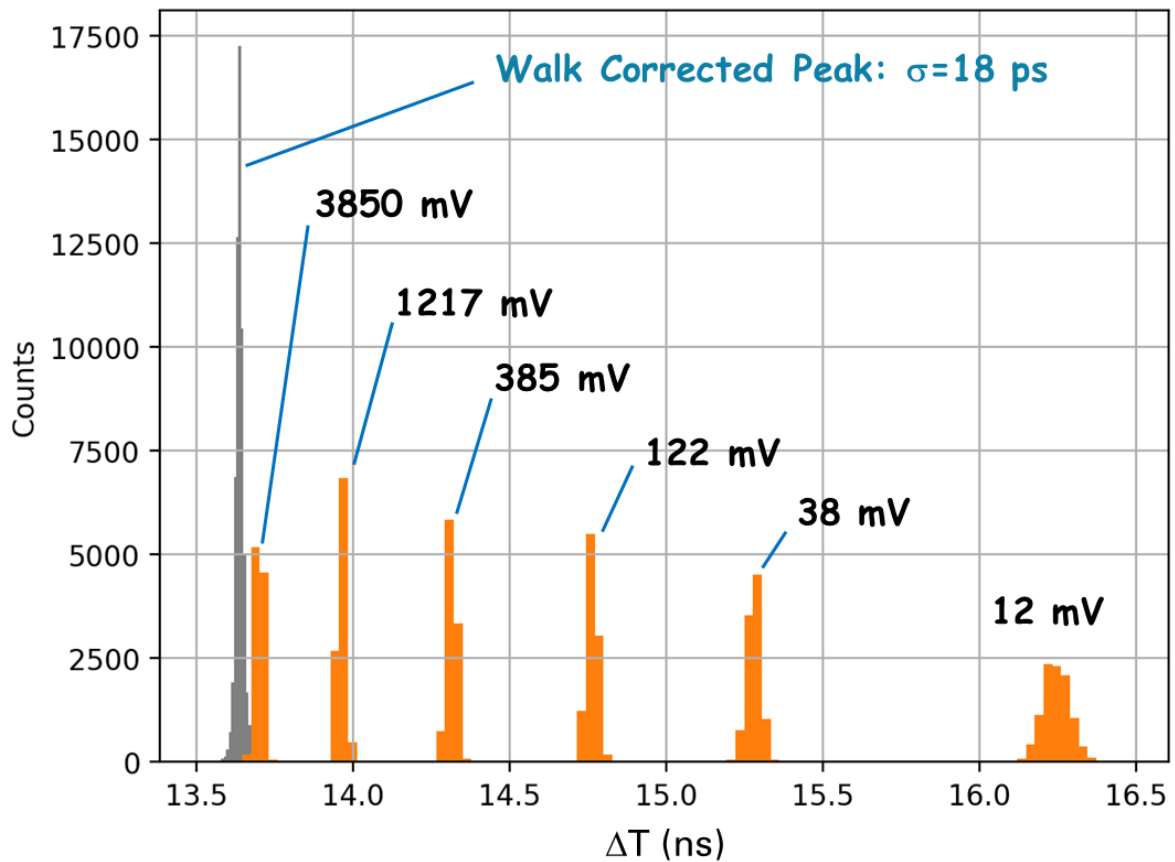
Fig.2 ToA measurements of input signals at different amplitudes before (orange) and after (grey) walk correction.
