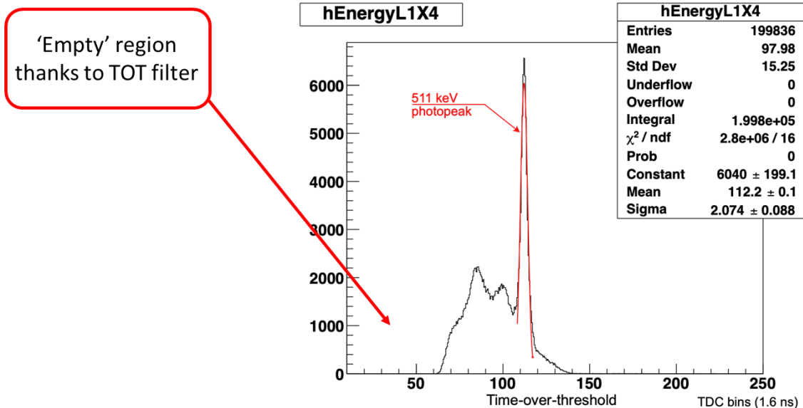
Fig.4 Na22 spectrum obtained via A5203 ToT measurements (ToT resolution of 1.6 ns). Noise reduction thanks to event suppression based on ToT threshold.
