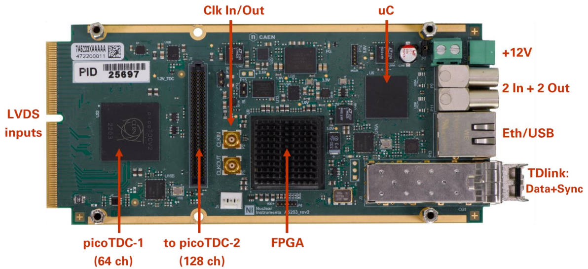
Fig.1 General view of the A5203 FERS unit, where the principal components and connectors are indicated.
