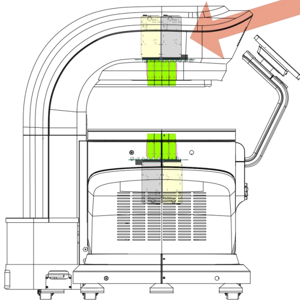
Fig.3 Positioning of A5203 units inside the ProVision PET scanner.
