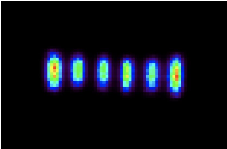
Fig.5 Coronal view of a stack of 6 Na22 sources obtained during tests of the Picotech PET scanner.
