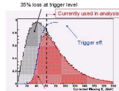
Figure 12: Expected signal shape as a function of corrected E_T of the SM Higgs assuming M_H = 120 GeV for the Higgs search in the ZH \rightarrow \nu\nu b\bar{b} channel. The blue curve shows the efficiency of the trigger requiring MET and two jets currently used, and the red histogram shows the signal acceptance due to the trigger. Approximately 50% of the signal is lost after applying an offline cut to avoid systematic uncertainties in the trigger turn-on.
