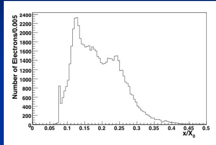
Fraction of a radiation length traversed by leptons from W decay (CDF Wmass analysis)- \ll 1 X_0
