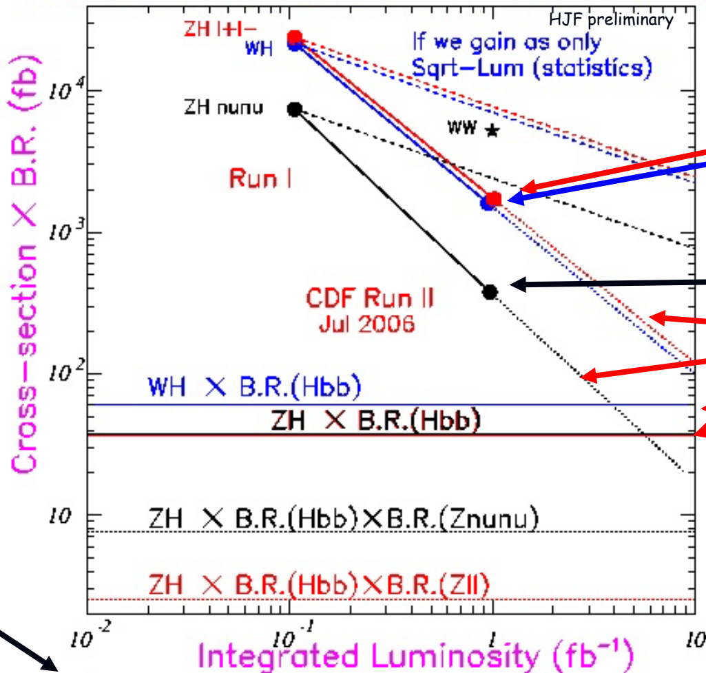
The Are We Getting Smarter? Plot 1 95% C.L. Limits on Cross-section \times B.R. M_H = 130 GeV
