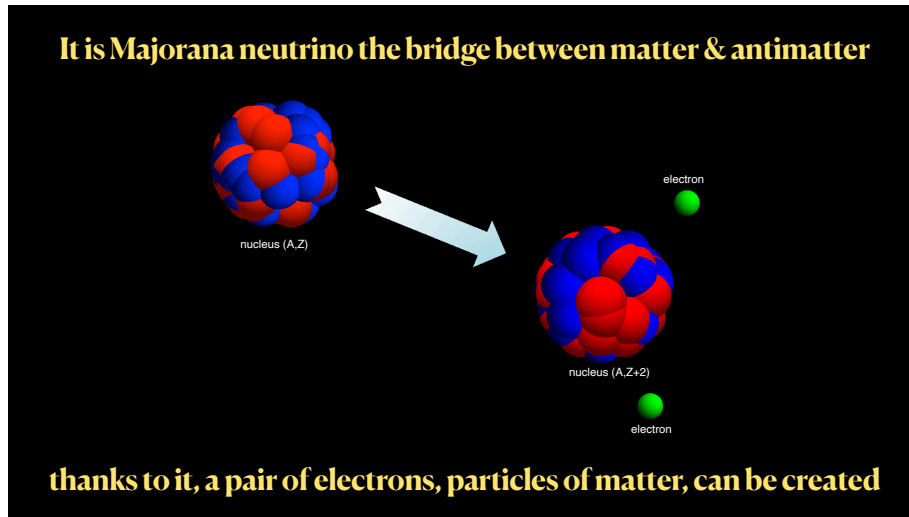
Figure 2: Illustration of the hypothetical nuclear transformation in which two of the neutrons contained within a nucleus become two protons, and at the same time an electron pair is created. This transformation is allowed by Majorana's neutrino theory: the speed of the transformation is proportional to the square of the neutrino mass associated with the electron. It is the subject of passionate research in laboratories all over the world, including those at the Gran Sasso lab, which are at the forefront.
