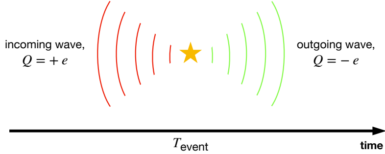
Figure 4: In Majorana's description of fermions and in any given space-time point, there is the possibility of emitting an electron wave (depicted in green), or of absorbing a positron wave (depicted in red). Imagine that in this space-time point there is a nucleus (the star); both situations will increase its electric charge by exactly one unit ( +e ). There is no need to think that the nucleus gains energy by emitting negative energy electron: it is enough to think that the gain is due to positron absorption.
