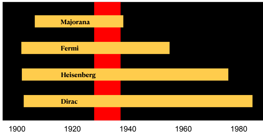
Figure 1: Comparison of the essential biographical data of Ettore Majorana and three scientists, who have been particularly important to him. The red band indicates the period in which Majorana published the three works described in the text.
