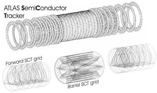
Figure 1: The layout of the silicon detector modules in the ATLAS SemiConductor Tracker. The three SCT sections are monitored using FSI geodetic grids. Each of the 842 lines represents an interferometric distance measurement between grid nodes. The SCT is 5.6m long.
