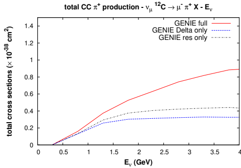
Figure 2.13: \pi^+ total cross section resulting from \nu_\mu^{12}C interactions. Different lines show results including all sources, all resonances, and the \Delta resonance alone. The nonresonant processes are significant in GENIE.
