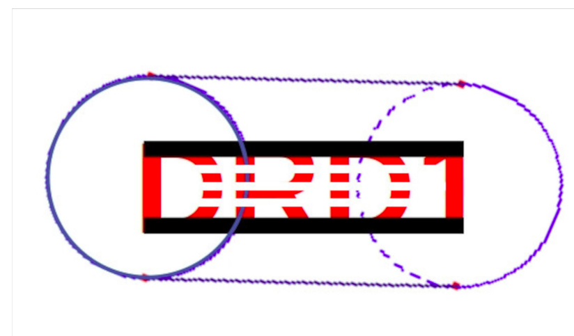
A cylinder to represent a TPC with the DRD1 text between 2 electrodes symbolising RPC or GEM. DRD1 letters not continuous to illustrate multigap RPC or mesh grid.
