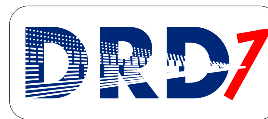
DRD text with different patterns (wire strip dots or RPC MPGD wires... whatever) and the 1 is an ionisation track with ionisation starting in the middle ...connected to the strips... ;-)
