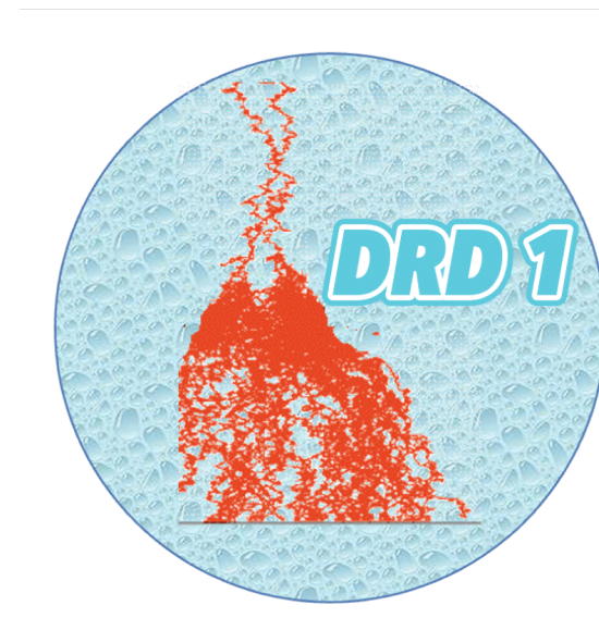
Avalanche as the common term between technologies given the wide variety of detector designs in collaboration
