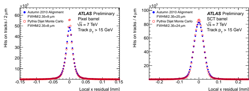
Figure 1: The Pixel and SCT local x residual distributions for the jet trigger data sample reconstructed with the Autumn 2010 Alignment (full circles), compared with the dijet MC simulation sample (open circles). The distributions are integrated over all hits-on-tracks in barrel modules and tracks are required to have p_T > 15 \text{ GeV} .
