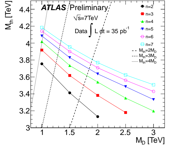
Figure 2: Contour plots of observed limits on Planck scale ( M_D ) versus threshold mass ( M_{th} ) [2].
