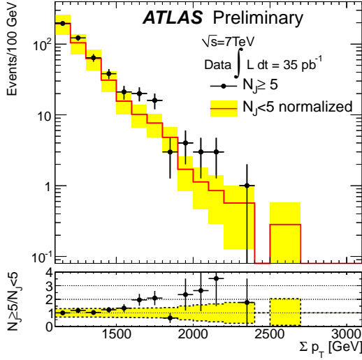
Figure 1: The \Sigma p_T distribution of the data. The points and histogram show the events with N_J \geq 5 and N_J < 5 , respectively [2].
