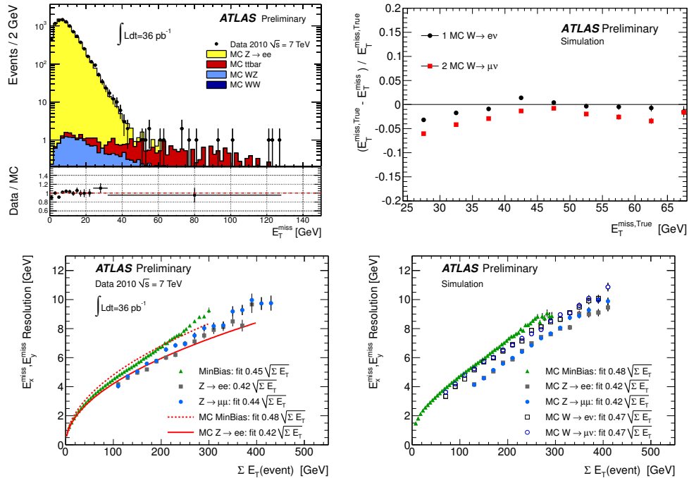
Figure 1: Main results for the E_T^{\text{miss}} performance in 2010 data (left plots) and in MC simulation (right plots). Further details in the text.
