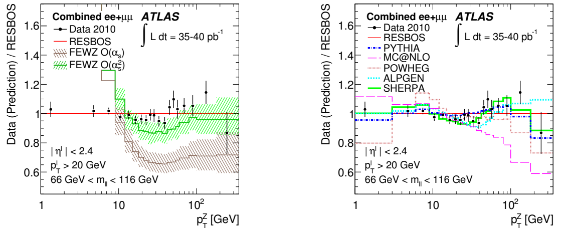
Figure 1: Ratios of the combined data and various predictions over the RESBOS prediction for the normalized differential cross section as a function of p_T^Z . Left: FEWZ predictions at \mathcal{O}(\alpha_s) and \mathcal{O}(\alpha_s^2) ; right: predictions from the generators PYTHIA, MC@NLO, POWHEG, ALPGEN, and SHERPA. The FEWZ predictions are shown with combined scale, \alpha_s , and PDF uncertainties. The data points are shown with combined statistical and systematic uncertainty. At low p_T^Z the \mathcal{O}(\alpha_s) and \mathcal{O}(\alpha_s^2) predictions of FEWZ diverge and are omitted.
