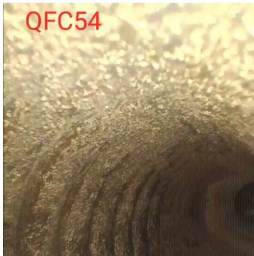
Cu erosion due to high water speed (8 to 14 m/s)
