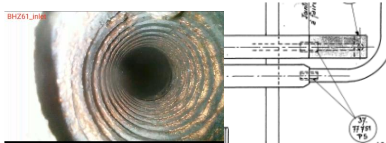
Brazed insert between busbar and coil (Sil-fos)
