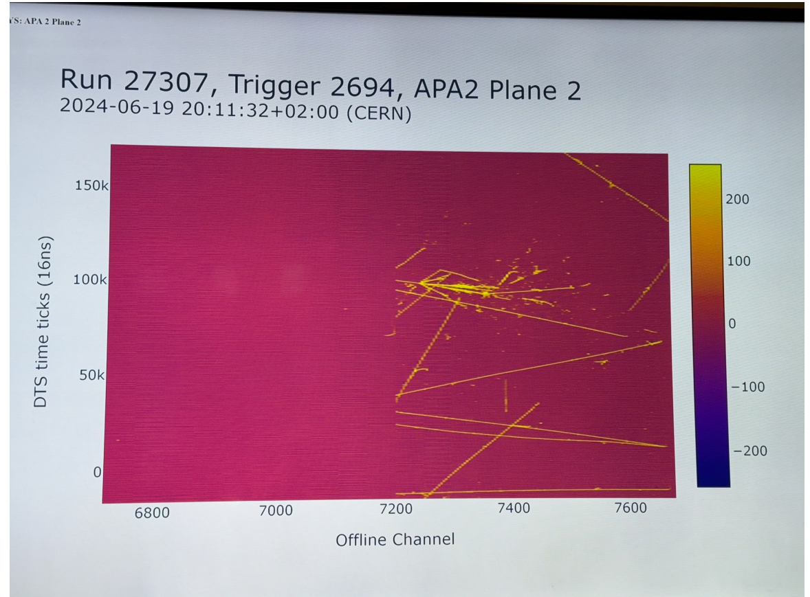
Pion interacting after \sim 3\text{m} in LAr
