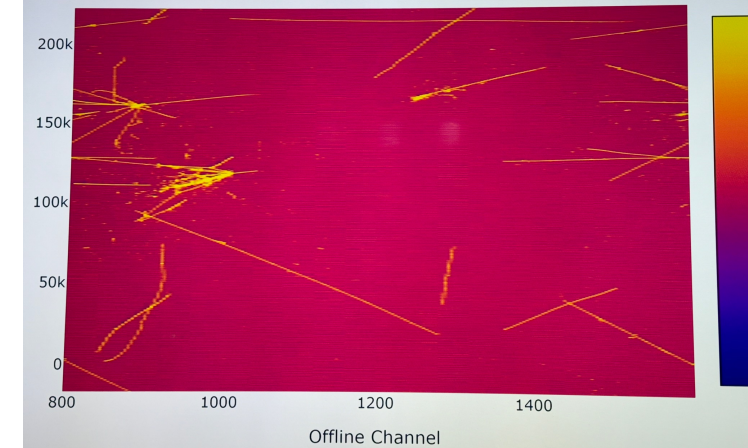
Run 27305, Trigger 1732, APA1 Plane 1 2024-06-19 19:39:35+02:00 (CERN)
