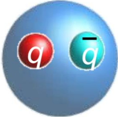
Charmonium
