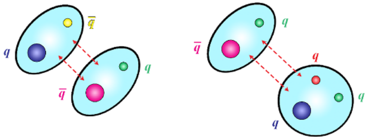
(g) weakly-bound hadronic molecules
