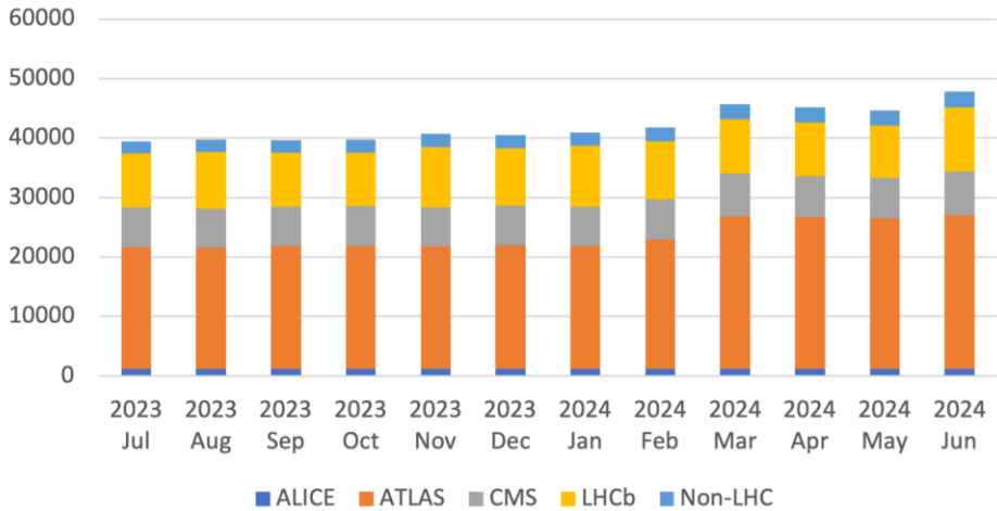
Disk Usage
