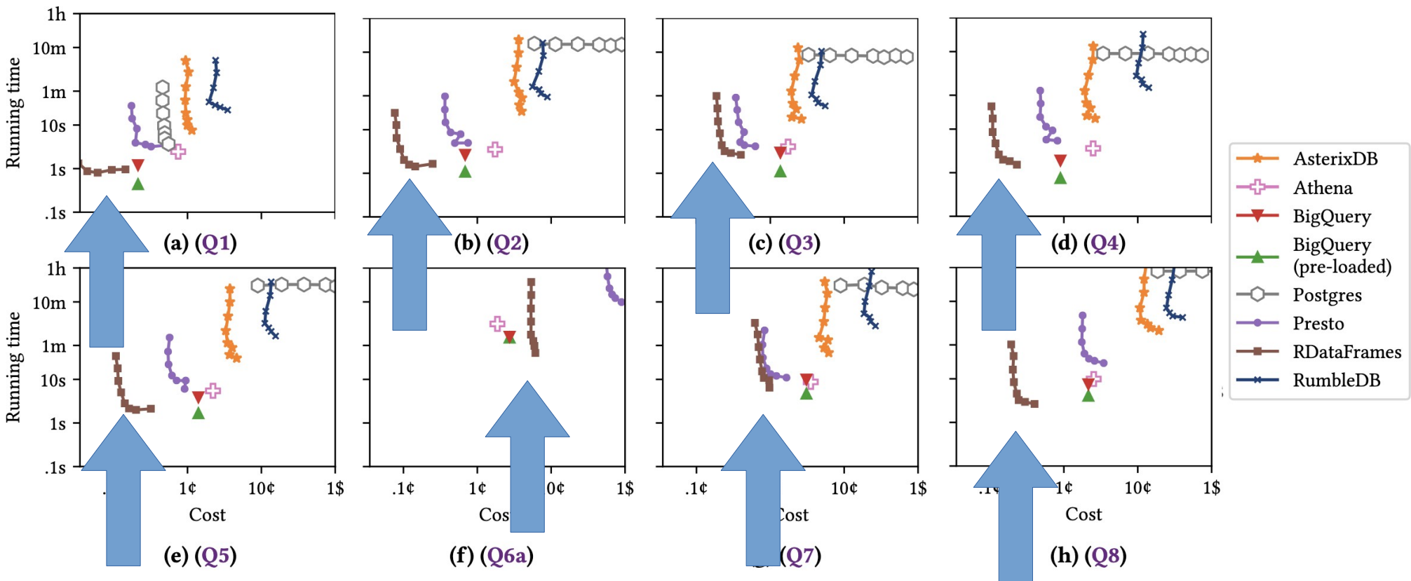
Figure 1: Running time/cost trade-off for various systems under test.
