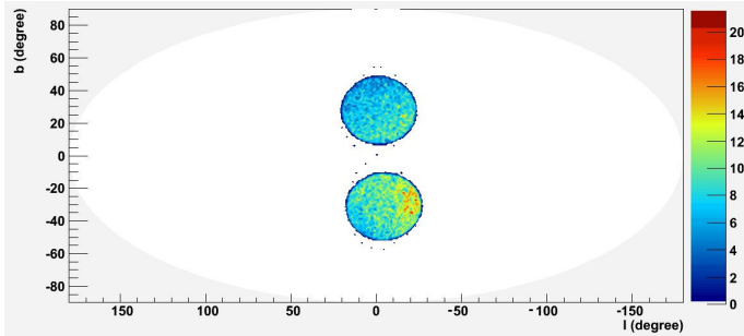
Figure 1: MC events generated up-going in galactic coordinates. The measured [4] bubble edges are also reported (points)
