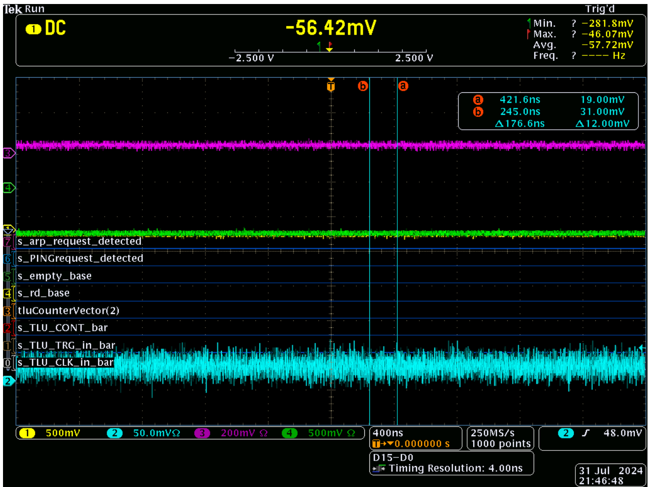
Figure 1: GND Piggy; Power Off
