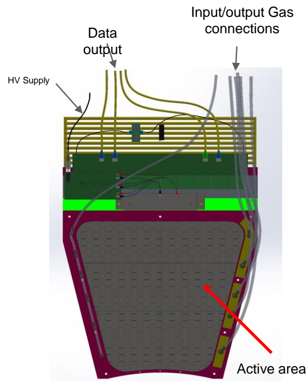
Module Front View with Components
