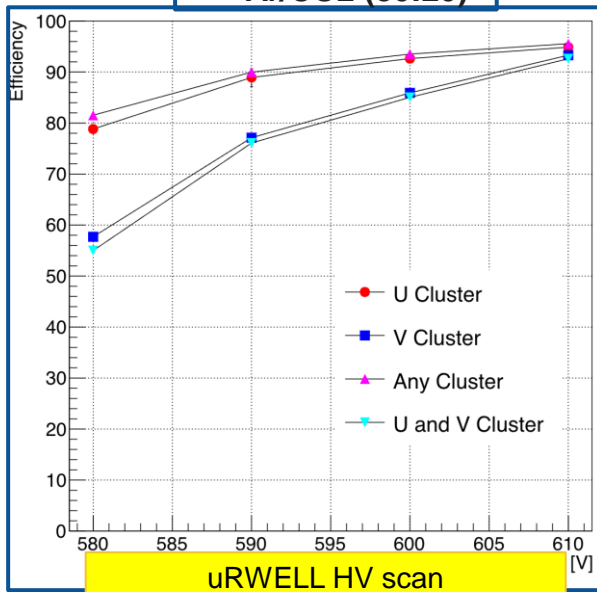
Ar/CO 2 (80:20)
