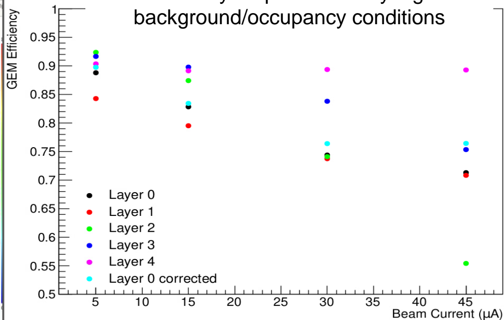
Efficiency vs. Beam Current
