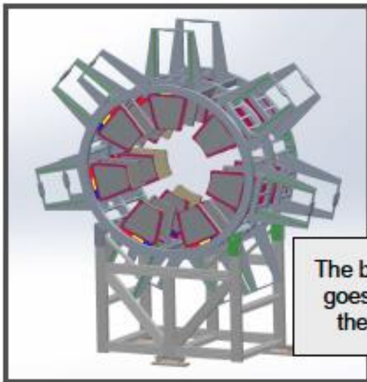
GEM Module Rotator Orientation during Calibration runs
