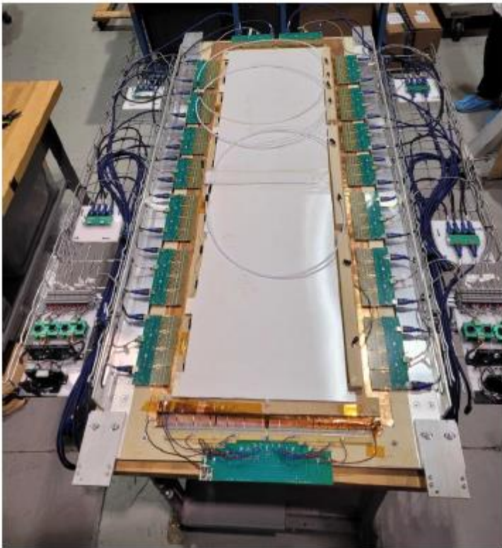
UV (shown) 40 x 150 sq.cm Single module
