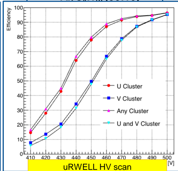
Ar/C 4 H 10 (90:10)
