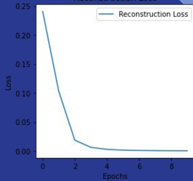
Reconstruction Loss
