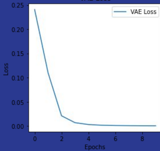
VAE Loss
