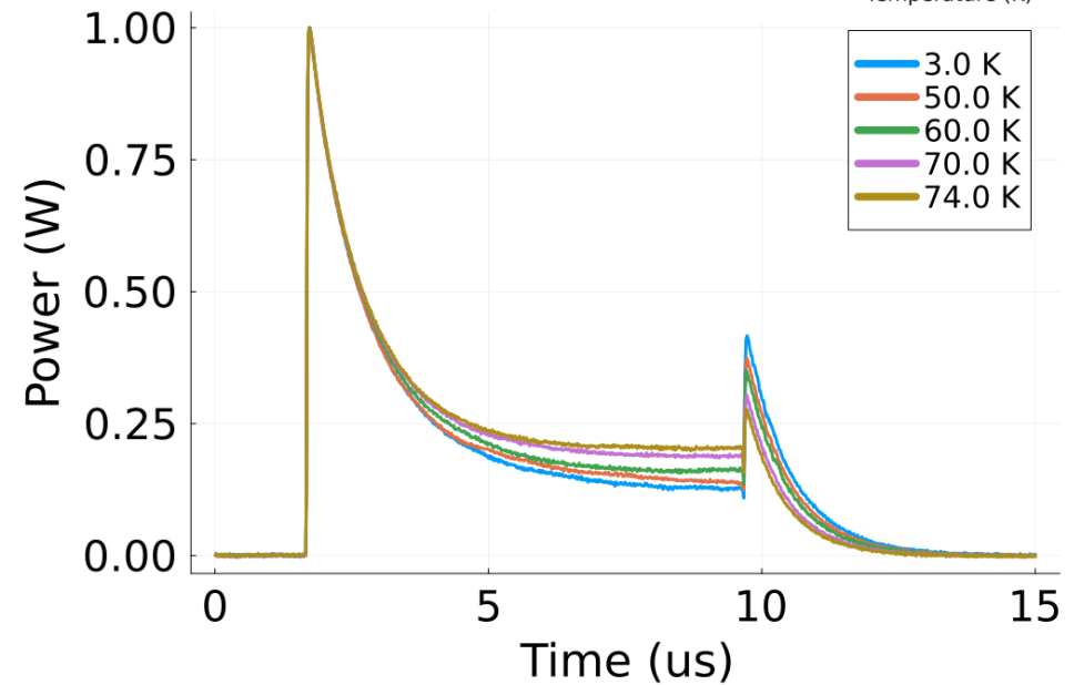
GdBCO Quench at 1700 W
