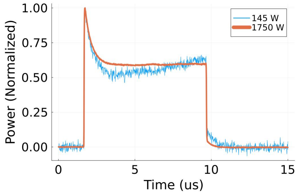
BSCCO Quench at 30 K
