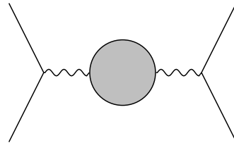
SILH basis
