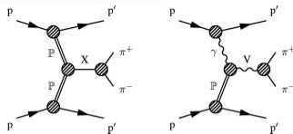
Central Exclusive Production
