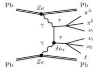
di- \tau production
