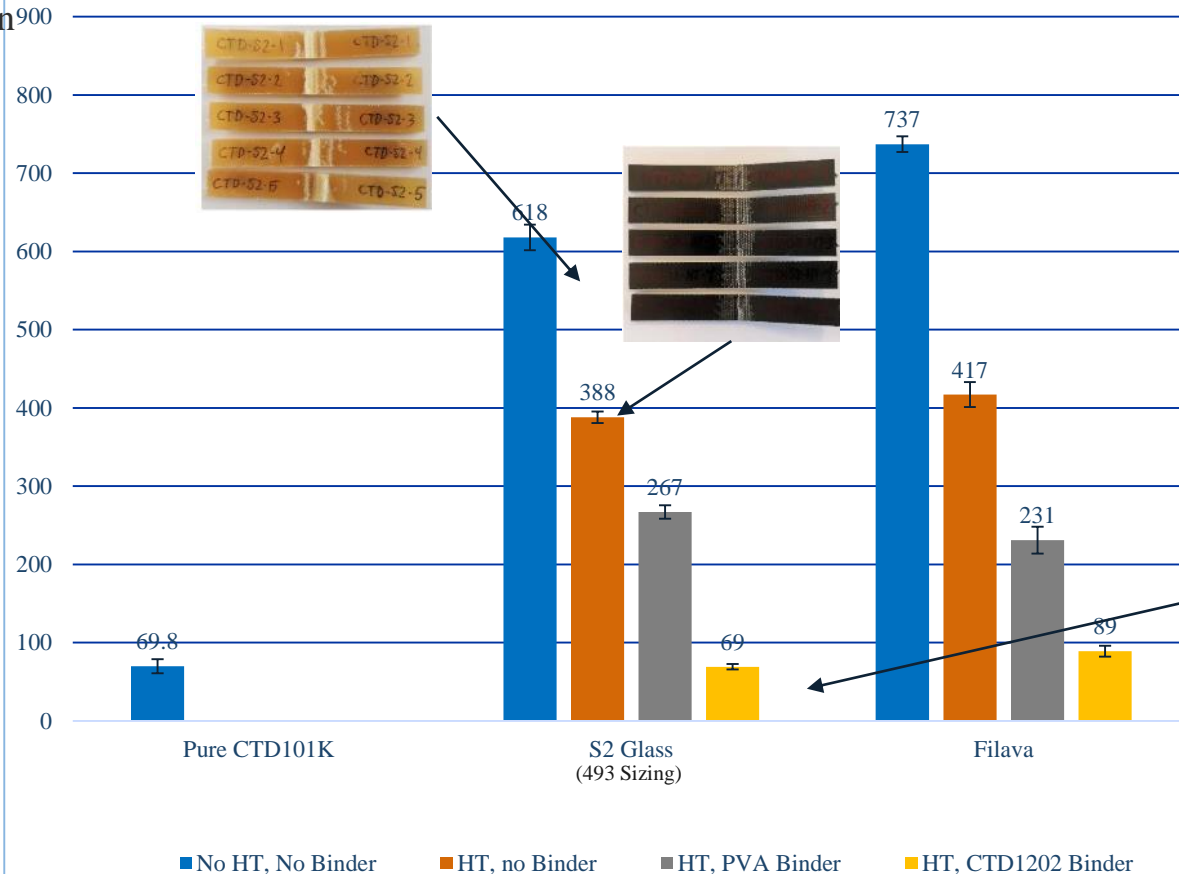
Flexural Strength (MPa)
