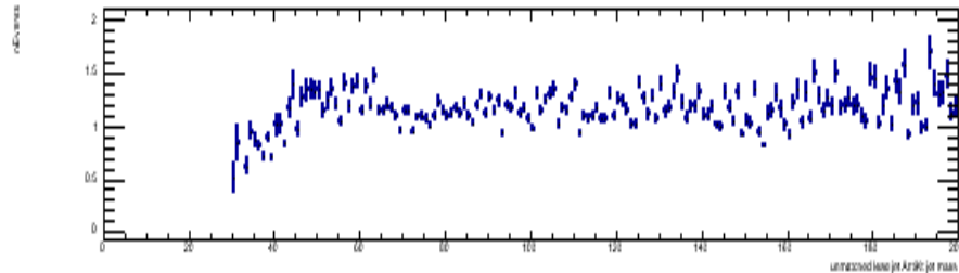
mass of CamKt filtered jet
