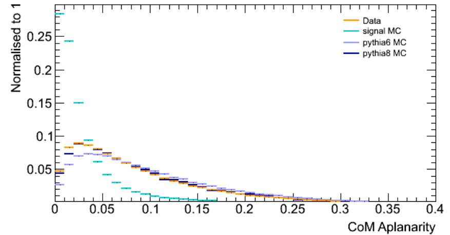
com aplanarity
