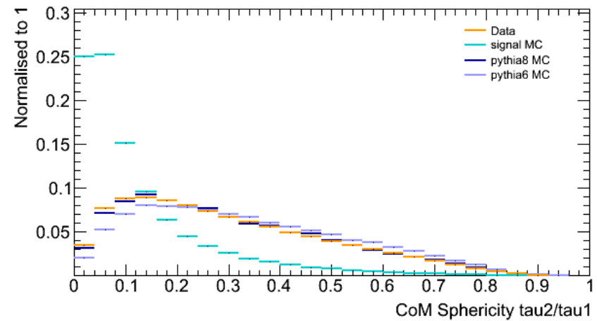
com sphericity
