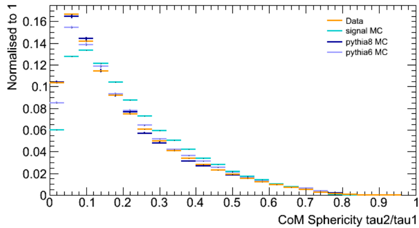
com sphericity
