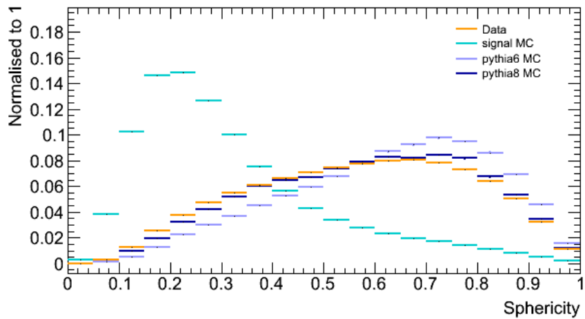
sphericity
