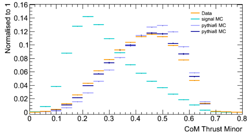
com thrust minor
