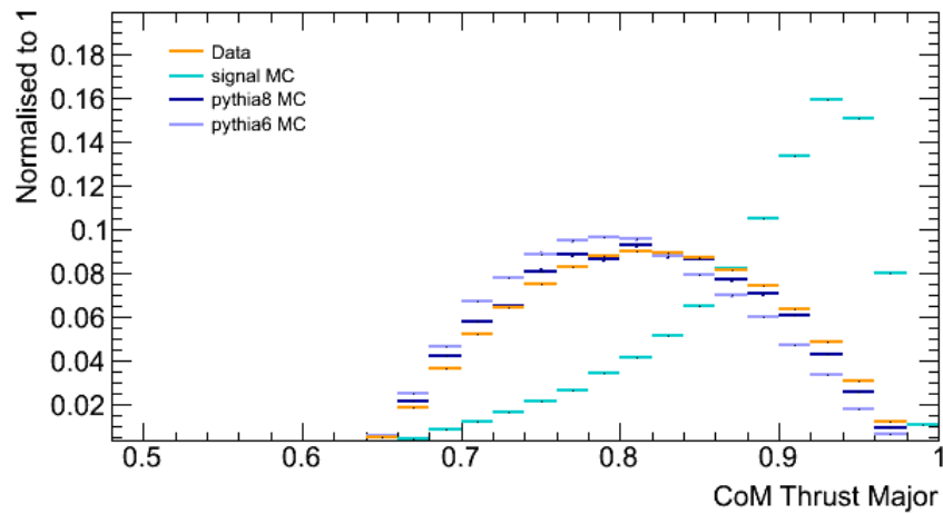
com thrust major
