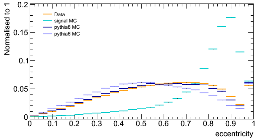
eccentric
