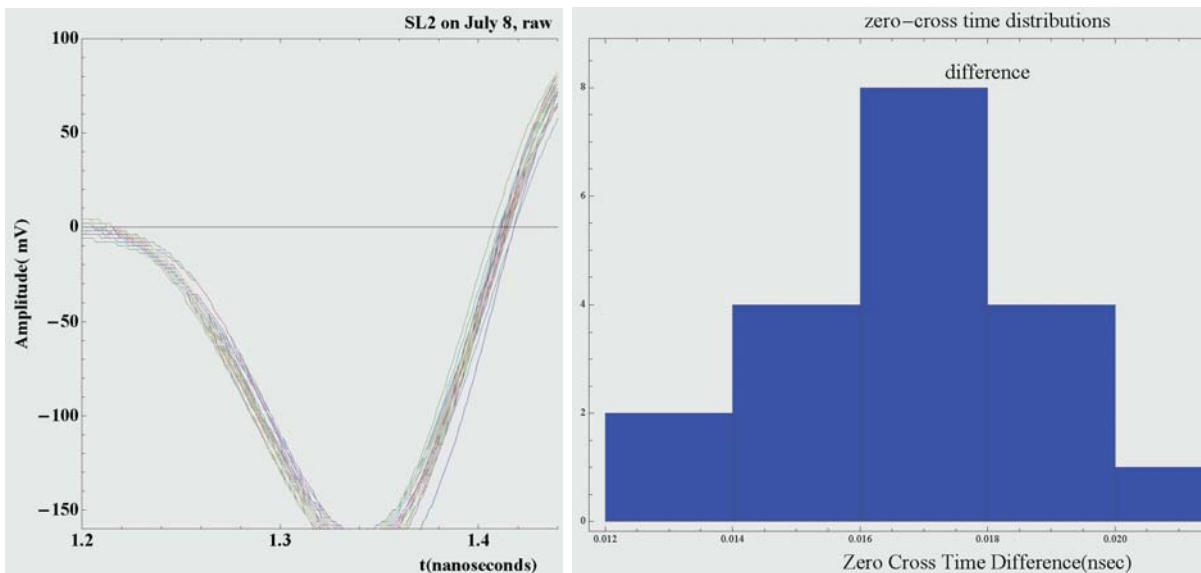
Figure 2: Left: Scope traces of signals from the electron beam of the BNL AFT. Right: Histogram of the zero crossing of the signals, with 2.5 ps (rms). Data collected July 8, 2010, by the BNL collaborators on the present proposal.
