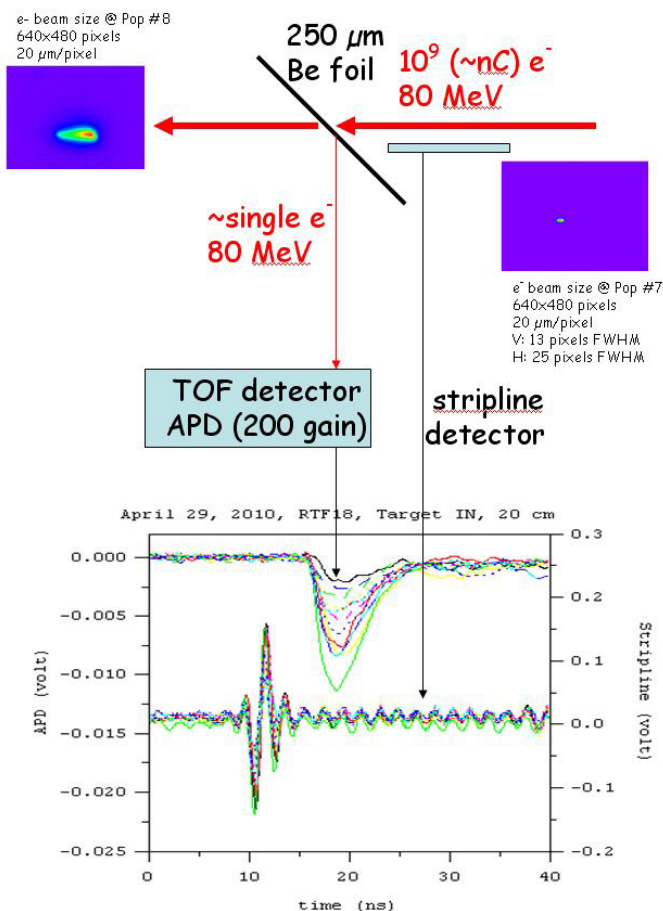
Figure 3: Schematic of the 80-MeV, single-electron test beam at the BNL Accelerator Test Facility. Single electrons are scattered by 90^\circ by a Be foil. A fast-timing trigger is provided by the stripline monitor of the pulse of 10^9 electrons in the primary beam. From 11 .
