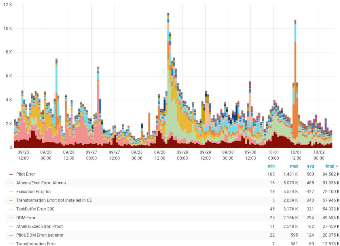
Panda Failure Categories - Stacked Bar Graph
