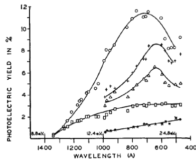
FIG. 2. Photoelectric yield of Ni. O Untreated cathode. □ Heat treated cathode in equilibrium with residual gases at about 10 -3 mm Hg. * Cathode maintained at 900°C in a vacuum of 10 -5 mm Hg. Δ Heat treated cathode at room temperature after exposure to O 2 at 0.1 mm Hg for one-half hour. + Heat treated cathode, heated in 0.05 mm Hg of O 2 at 800°C for one minute.
