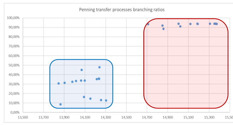
BR and excited state population at 100mb
