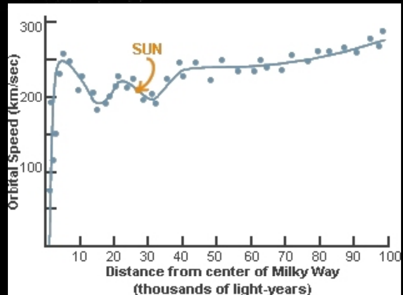
Milky Way
