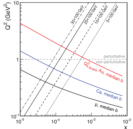
Figure 1: Kinematic coverage in x and Q^2 of the EIC for different beam energies, compared with predictions of the saturation scale, Q_s^2 , in p , Ca , and Au .
