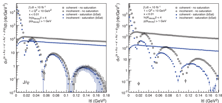
Figure 3: d\sigma/dt distributions for exclusive J/\psi (left) and \phi (right) production in coherent and incoherent events in diffractive eA collisions. Predictions from saturation and non-saturation models are shown.
