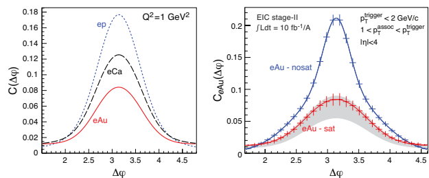
Figure 2: Saturation model [10] predictions of azimuthal angle difference ( \Delta\varphi ) between two hadrons in ep , eCa , and eAu (left), and comparisons with calculations from conventional non-saturated model (right).
