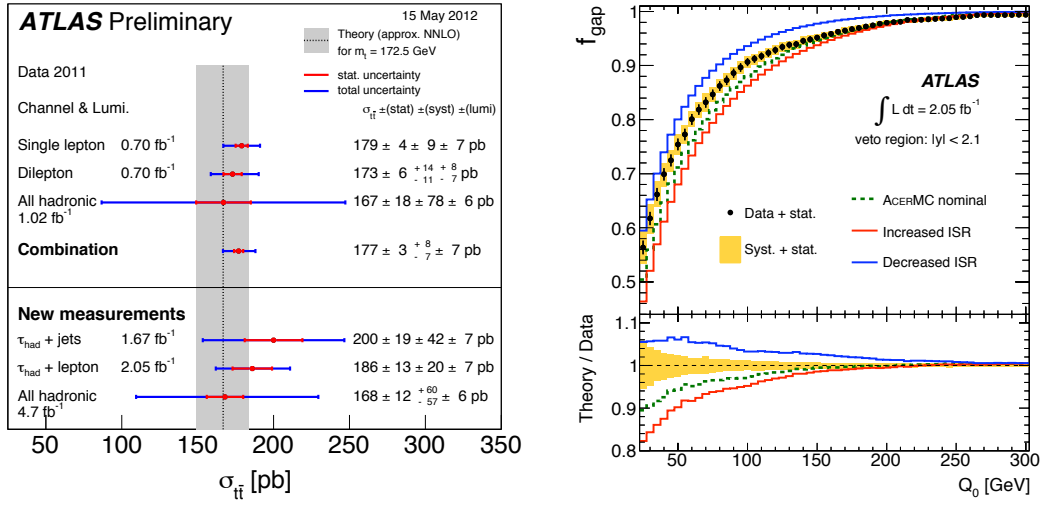
Figure 1: The left plot [3][13] shows a summary of \sigma_{t\bar{t}} measurements compared to the theoretical expectation, including the individual and combined measurements (upper part) and the new measurements (lower part) including the \tau_{\text{had}} + \text{lepton} [14] channel. The right plot [9] shows the measured f(Q_0) compared with the ACERMC prediction, where PYTHIA parton shower parameters are varied to produce samples with nominal, increased and decreased ISR.
