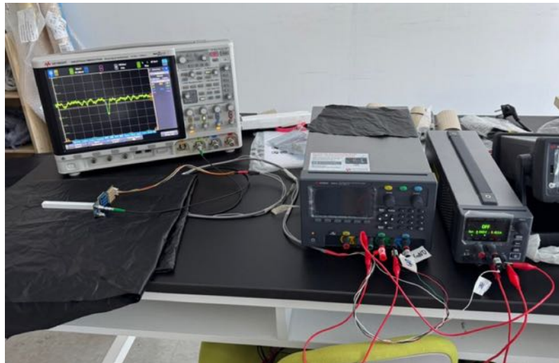
SiPM board (S13361-6050AE-04)
