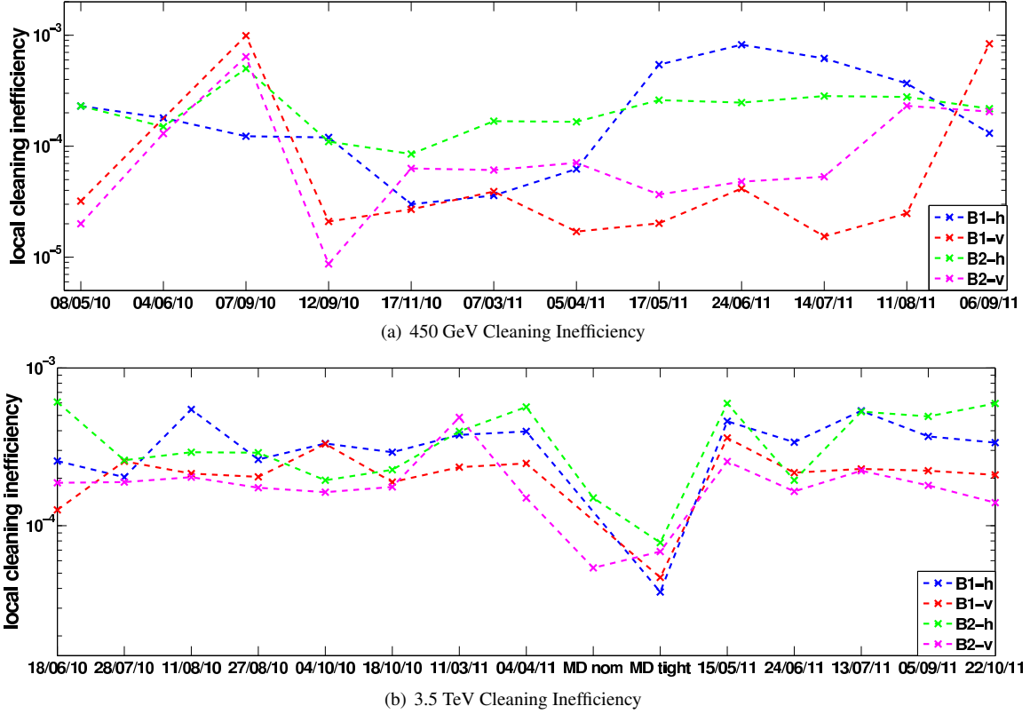
Figure 6: Proton cleaning inefficiency throughout 2010 and 2011. The inefficiency remains constant except for when nominal and tight collimator settings were used during MDs.
